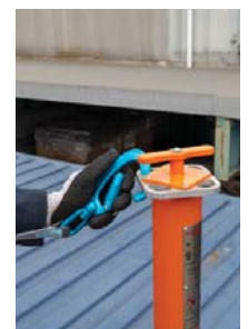
Attach hook on SRL to anchor point on container post
